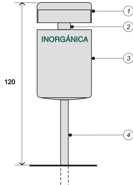
VISTA FRONTAL
