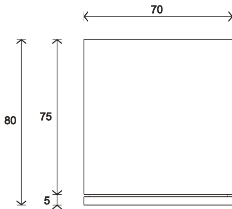
VISTA FRONTAL
