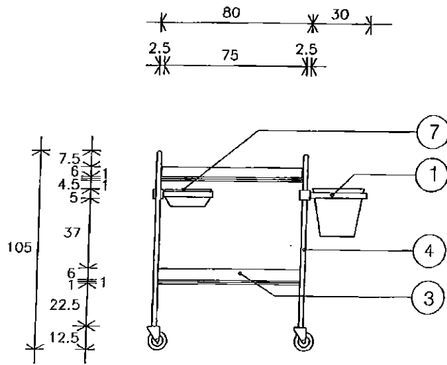
VISTA FRONTAL
